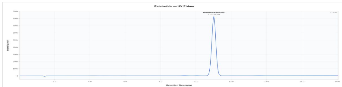
Retatrutide 60mg - 032026: UV Chromatogram
