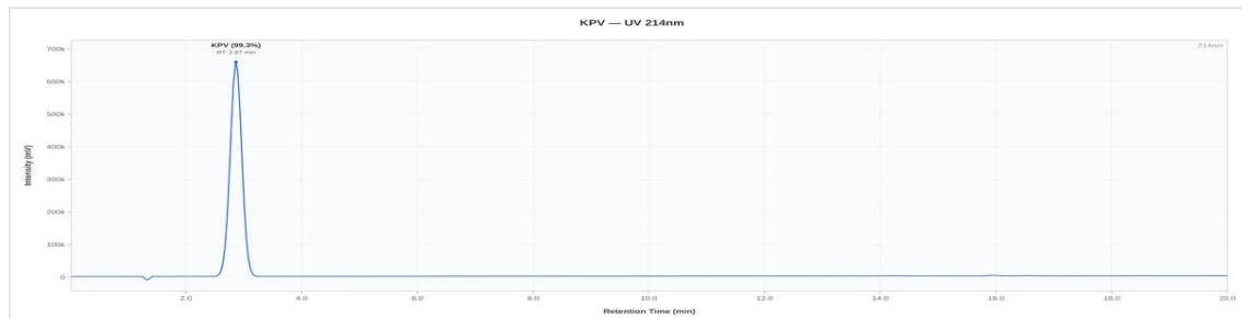
KPV 10mg - 032026: UV Chromatogram
