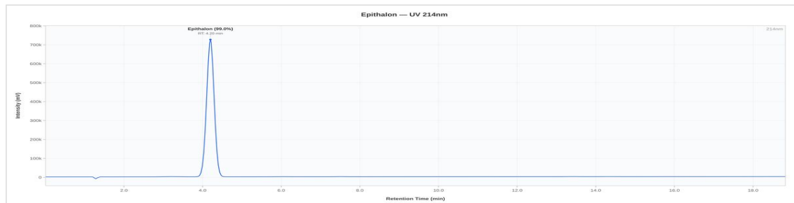
Epithalon 10mg - 032026: UV Chromatogram
