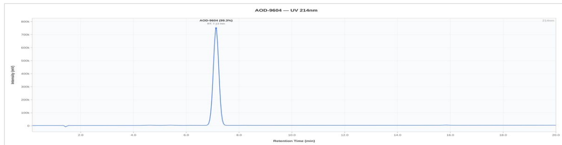
AOD-9604 5mg - 032026: UV Chromatogram
